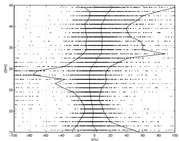
Figure 3. Relative differences ( 100 \cdot (\text{ACE} - \text{GOMOS}) / \text{GOMOS} ) of all O_3 profiles. The thin line is the median value and the thick lines refer to the 0.16 and 0.84 percentiles of the distribution.
