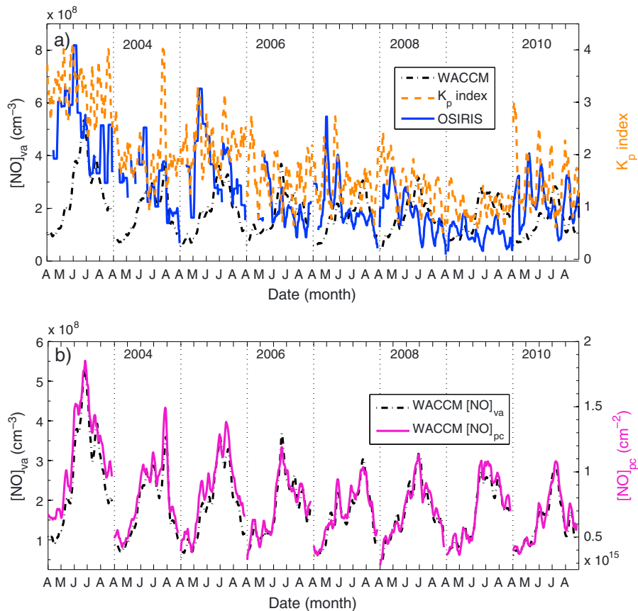
Figure 4. (a) Comparison between OSIRIS (same conditions as Figure 2) and 10 day mean SD-WACCM [\text{NO}]_{va} and 10 day averaged 3 h K_p index values. (b) 10 day mean SD-WACCM [\text{NO}]_{va} compared with SD-WACCM [\text{NO}]_{pc} (partial column densities from 50 to 130 km).
