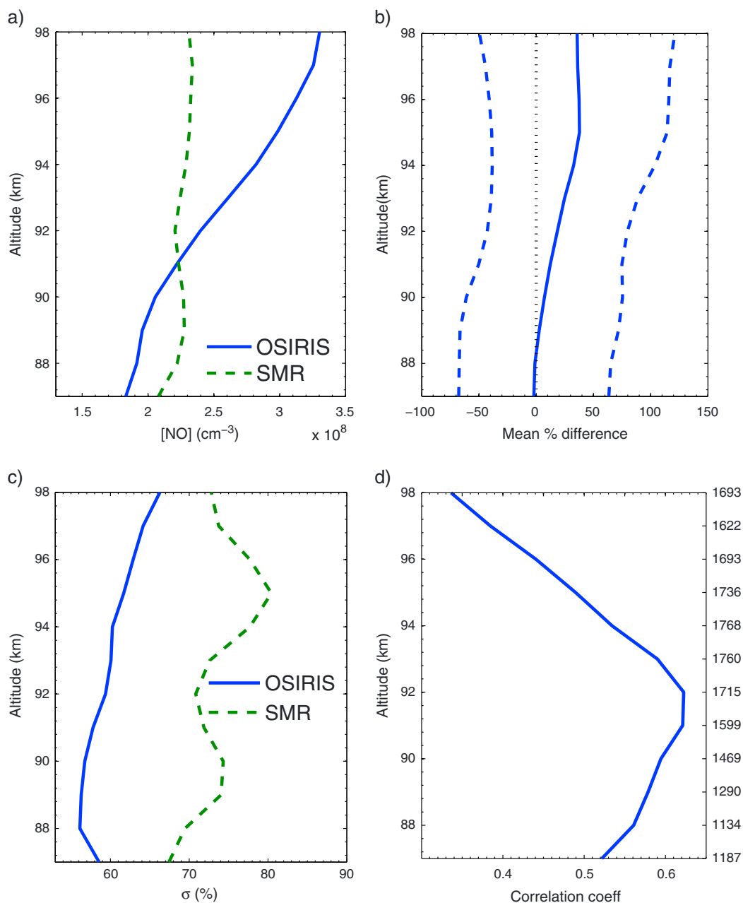
Figure 5. Statistical analysis of coincident OSIRIS and SMR profiles. OSIRIS profiles have been vertically smoothed using the 7 km running mean, and coincident profiles where the OSIRIS values are negative have been excluded. (a) Mean coincident OSIRIS and SMR [NO] profiles. (b) Mean percent difference profiles, 100% (OSIRIS – SMR) / mean, dashed lines indicate the \pm 1\sigma standard deviation. (c) OSIRIS and SMR measurement standard deviations. (d) Correlation coefficient profiles. Numbers on right-hand side indicate number of coincident retrievals at a given altitude.
