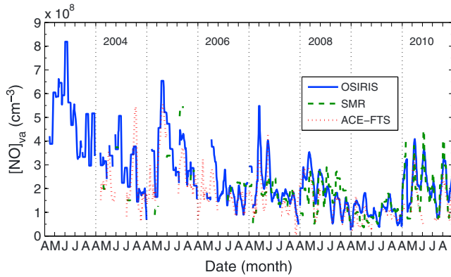
Figure 2. Comparison of OSIRIS, SMR, and ACE-FTS vertically averaged [NO] (vertically averaged between 90 and 100 km) for days 91–244 of each year. Both AM and PM data are included, and data are smoothed by the 10 day running mean.
