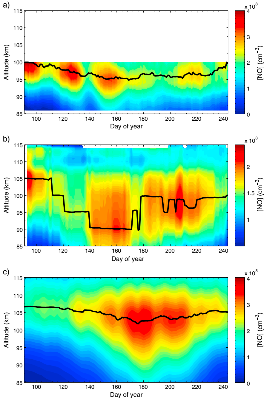
Figure 6. Antarctic [NO] climatologies for 2003–2010 from (a) OSIRIS, (b) SMR, and (c) SD-WACCM. The OSIRIS and SD-WACCM data are smoothed by their respective 10 day running means, whereas the SMR data are smoothed by the 30 day running mean. The solid black lines indicate the [NO] peak altitude.
