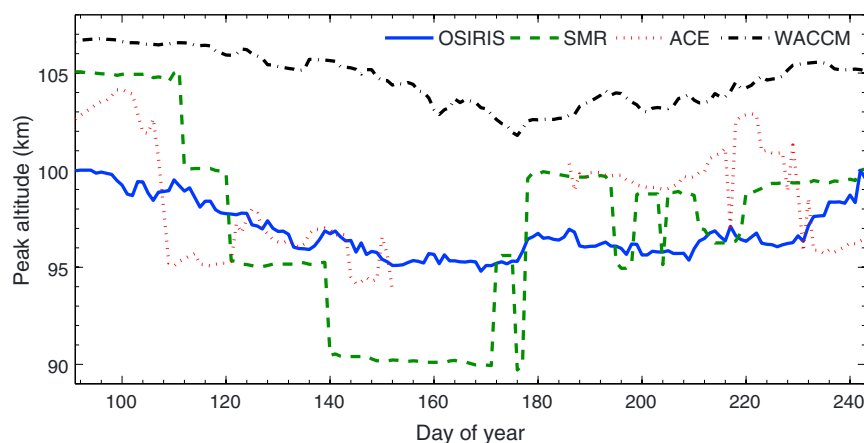
Figure 8. Peak heights of the satellite-derived and modeled NO climatologies. The SMR data were smoothed by the 30 day running mean, and all other data were smoothed by the respective 10 day running means.
