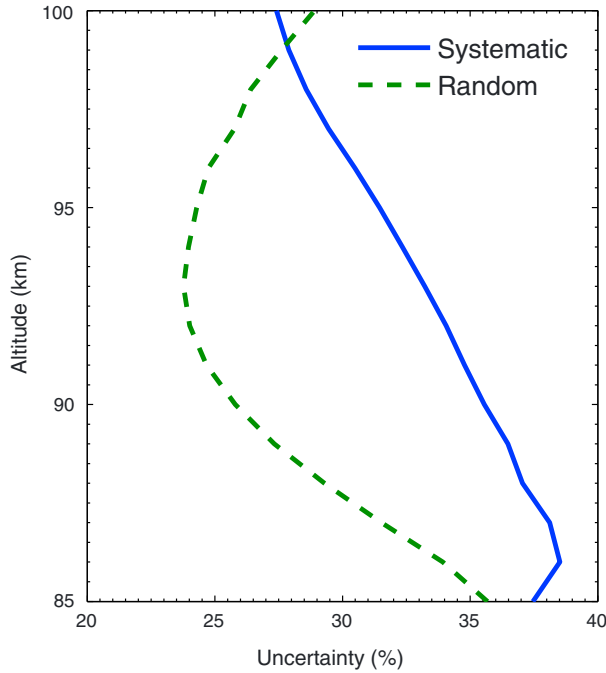
Figure 1. Systematic uncertainty and mean random uncertainty due to instrument noise in the OSIRIS [NO] profiles.
