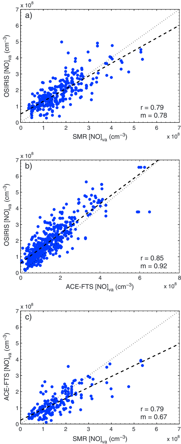
Figure 3. Correlation plots comparing three-day mean [NO] va values between (a) SMR and OSIRIS, (b) ACE-FTS and OSIRIS, and (c) SMR and ACE-FTS. Dashed lines are the linear fits, and dotted lines are the 1-to-1 line. Correlation coefficients, r , and slopes of the linear fits, m , are also shown.
