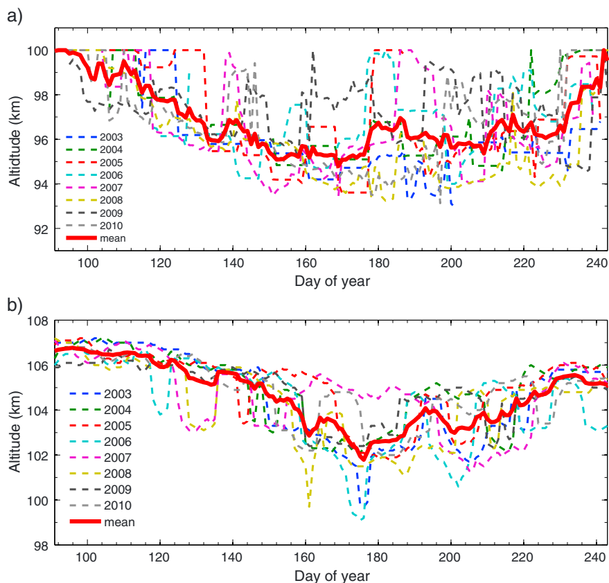
Figure 7. 2003–2010 climatological [NO] peak heights from (a) OSIRIS and (b) SD-WACCM.
