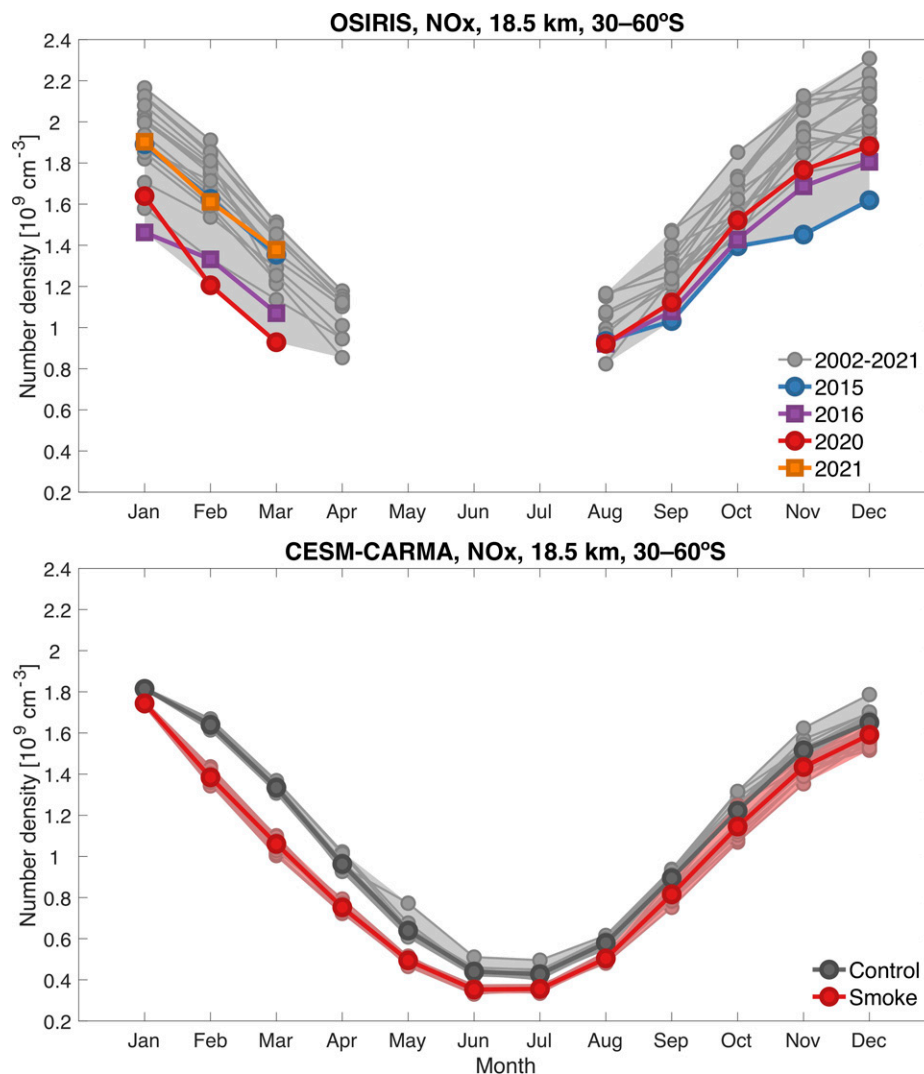
Fig. 3. NO x concentrations (molecules/centimeter 3 ) by month, averaged from 30 to 60°S at 18.5 km. The Top panel presents 20 y of OSIRIS measurements, with 2015 and 2016 (after the Calbuco eruption) and 2020 and 2021 (after the Australian black summer fires) distinguished from others by the indicated colors. The Bottom panel shows 20 realizations of 2020 both with (red) and without (gray) smoke for the same latitudes and altitude as calculated in the model.
