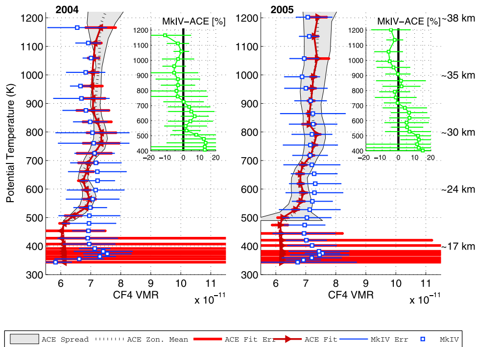
Figure 19. MkIV and ACE \text{CF}_4 comparisons. Details as for Figure 4.
