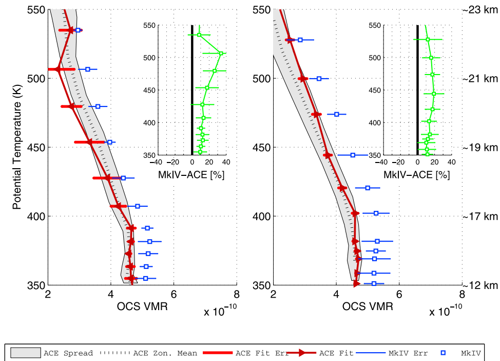
Figure 18. MkIV and ACE OCS comparisons. Details as for Figure 4.
