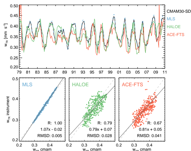
Figure 13. Top: w_{\text{TR}} (monthly vertical velocities) derived using daily time correlations of the water vapor tape recorder at different pressure levels from the raw CMAM30-SD data as well as the satellite-sampled data. w_{\text{TR}} derived using the raw model fields and MLS-sampled data are almost identical. The pressure levels averaged are 30, 40, 50 and 60 hPa. Bottom: w_{\text{TR}} scatterplots ( \text{mm s}^{-1} ) for MLS, HALOE and ACE-FTS sampling, respectively, vs. the velocities derived using raw model fields. The slopes' 95 % confidence intervals are \pm 0.007 , 0.06 and 0.09 for MLS, HALOE and ACE-FTS, respectively.
