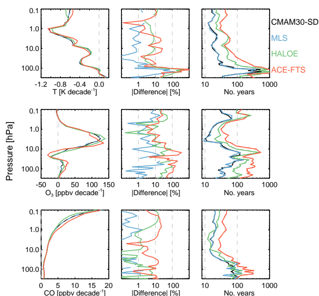
Figure 9. Left: near-global (60° S to 60° N) long-term (1979–2012) trends computed using Eq. (4) for temperature, \text{O}_3 and CO. Middle: percentage difference in the inferred magnitude of the trends when computed using various satellite-sampled data with respect to the one computed using the raw model fields. Right: number of years required to detect such trends.
