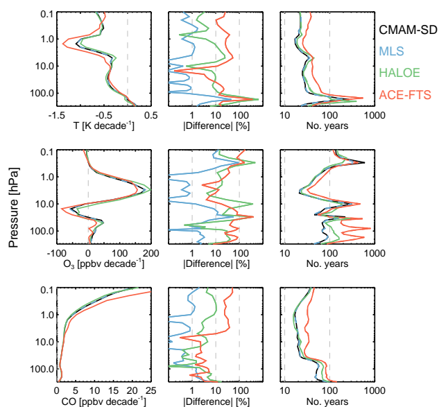
Figure 11. As Fig. 9 but for 30 to 60° N.
