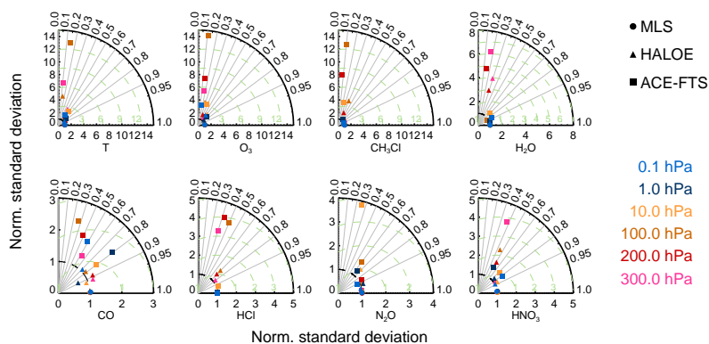
Figure 6. Taylor diagrams showing near-global (60° S to 60° N) long-term (1979–2012) pattern comparisons between the raw (the reference point at (1,0)) and the satellite-sampled data at different pressure levels. The green contours indicate the normalized RMS difference values.
