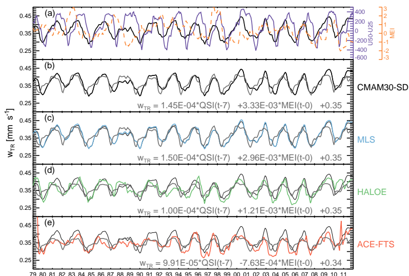
Figure 14. (a) Time series of w_{TR} (mean monthly vertical velocities averaged over 30, 40, 50 and 60 hPa) derived using CMAM30-SD raw data (black), the quasi-biennial oscillation (QBO) shear index (QSI – purple) and the multivariate ENSO index (MEI – orange dashed line). (b) Time series of w_{TR} for the raw model fields (black) as well as the model fit described by Eq. (10) (gray). (c–e) Time series of w_{TR} for satellite-sampled data (color coded). The thin black line displays the same w_{TR} derived using raw model fields (black line in b) for ease of comparison with the satellite-sampled ones. The model fit for each of the satellite-sampled w_{TR} values, described by Eq. (10), is shown in gray for each of these time series.
