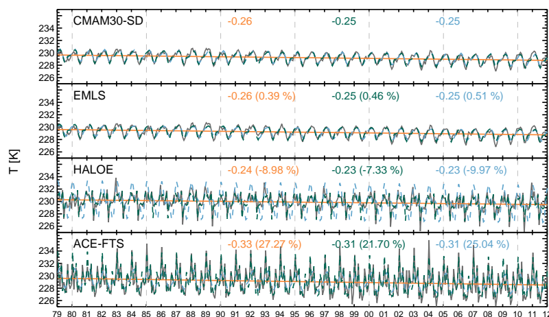
Figure 8. Time series of near-global (60° S to 60° N) temperature at 10 hPa for the raw and satellite-sampled data (gray lines). Orange lines display the trend computed using the linear fit, green lines show the climatological seasonal cycle imposed upon a long-term trend and light blue lines show the model computed using Eq. (4). The trend ( \text{K decade}^{-1} ) computed using each method is specified in each subplot; in brackets we show the percentage difference in trend magnitude with respect to the trend found using the raw model data.
