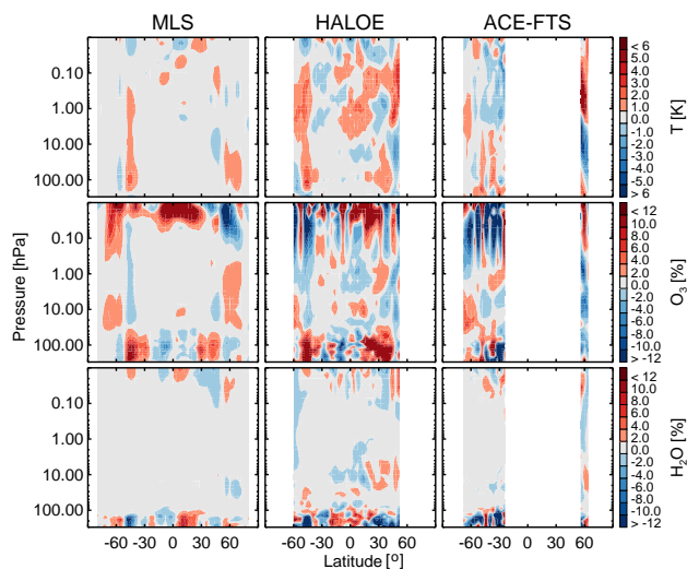
Figure 3. January 2005 sampling bias as a function of latitude and pressure for temperature, O_3 and H_2O (top to bottom) as measured using MLS, HALOE and ACE-FTS sampling patterns (left to right). White regions denote a lack of measurements.
