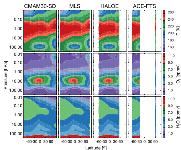
Figure 2. January 2005 zonal means as a function of pressure for temperature, O_3 and H_2O (top to bottom) in 4^\circ latitude bins. Left column is raw CMAM30-SD model fields; other columns are CMAM30-SD as sampled by MLS, HALOE and ACE-FTS (left to right), respectively. White regions denote a lack of measurements.
