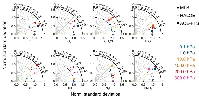
Figure 10. As Fig. 6 but for 30 to 60° N.
