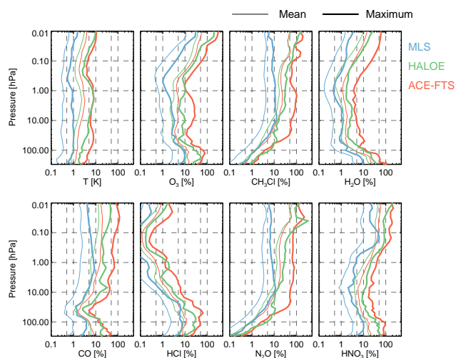
Figure 5. Mean (thin lines) and maximum (thicker lines) RMS sampling bias over all latitudes for 2005 as a function of pressure for temperature (in Kelvin), \text{O}_3 , \text{CH}_3\text{Cl} , \text{H}_2\text{O} , \text{CO} , \text{HCl} , \text{N}_2\text{O} and \text{HNO}_3 in percent. The vertical grid indicates values of 0.5, 1, 5, 10, 50 and 100.
