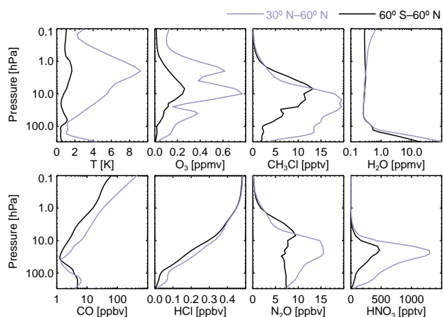
Figure 7. Raw model standard deviations used to normalize the Taylor diagrams shown in Figs. 6 and 10. Note that H 2 O and CO are shown using a logarithmic scale.
