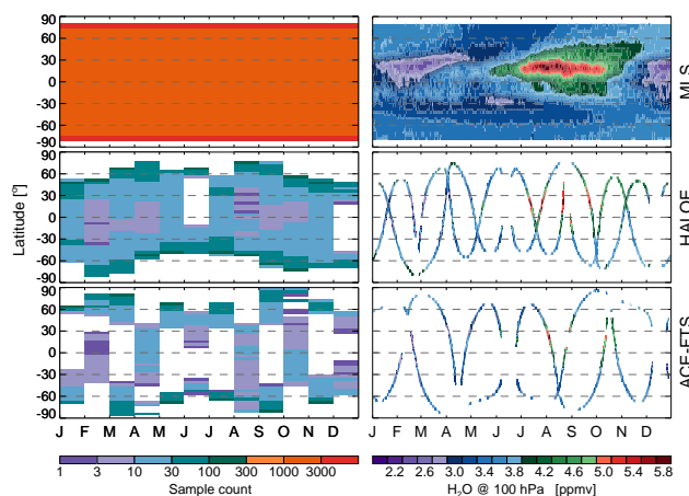
Figure 1. Left: monthly sampling counts for MLS, HALOE and ACE-FTS, in 4^\circ latitude bins. Note the nonuniform color bar increments. Right: zonal mean water vapor at 100 hPa as sampled by MLS, HALOE and ACE-FTS for individual days. White regions denote a lack of measurements.
