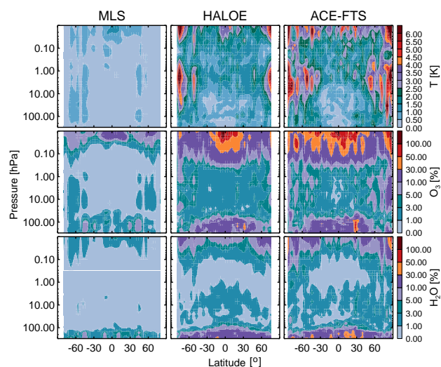
Figure 4. Root-mean-square sampling bias for 2005 as a function of latitude and pressure for temperature, O_3 and H_2O (top to bottom) as measured using MLS, HALOE and ACE-FTS sampling patterns (left to right). White regions denote a lack of measurements.
